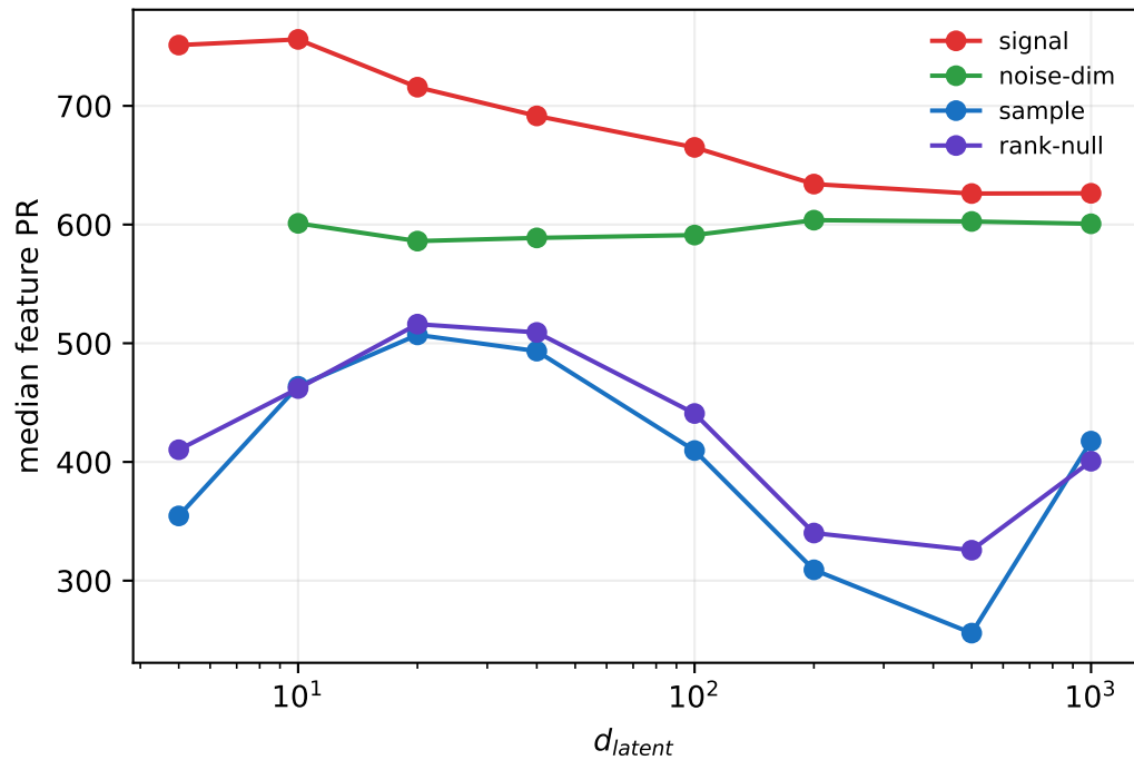
Feature-eigenvector participation ratio: p_fixed_energy_fixed
